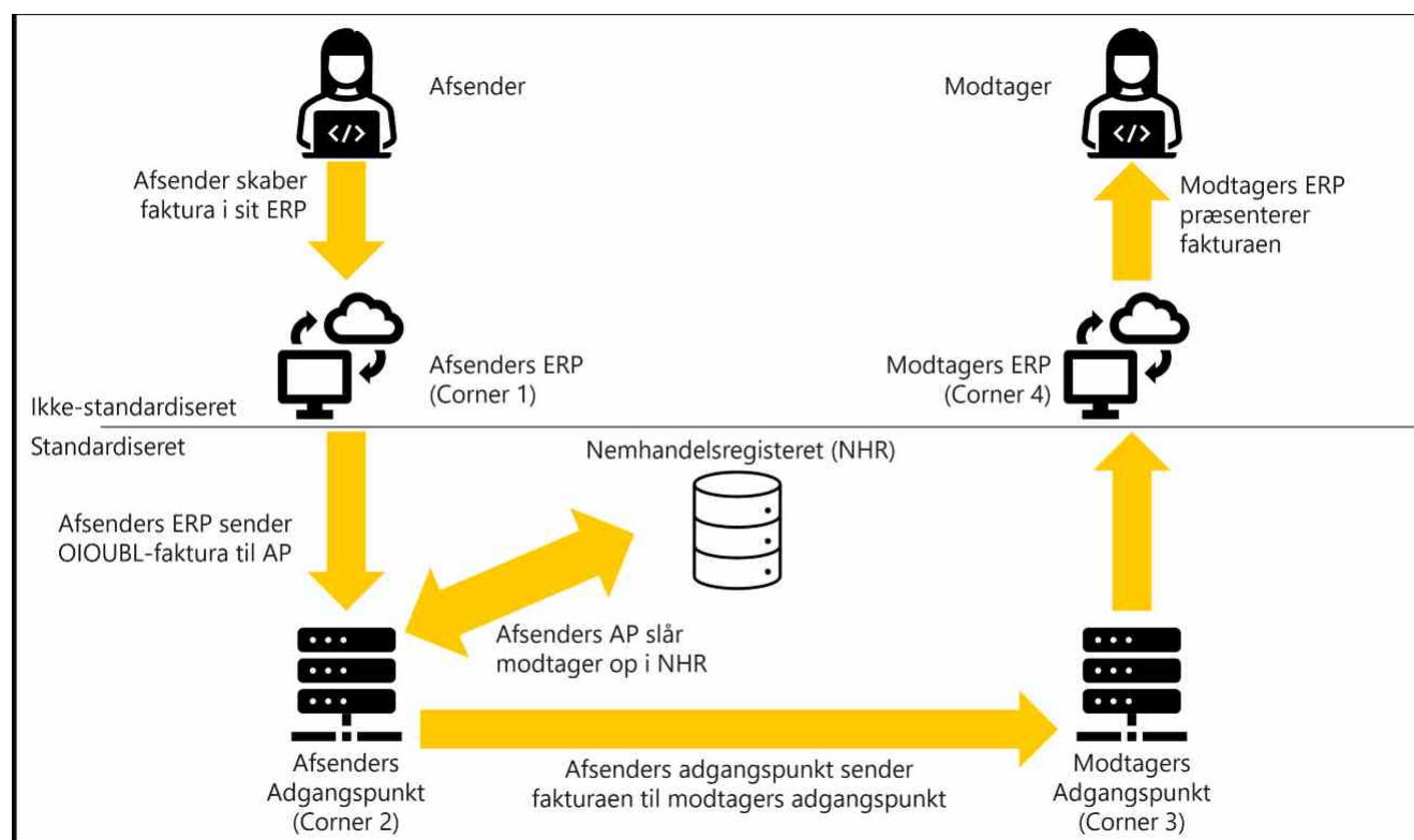
Figur 1: 4-corner model for Nemhandel eDelivery
